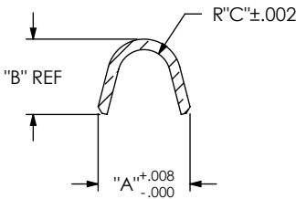
SECTION "A"- "A" SCALE 10 : 1
