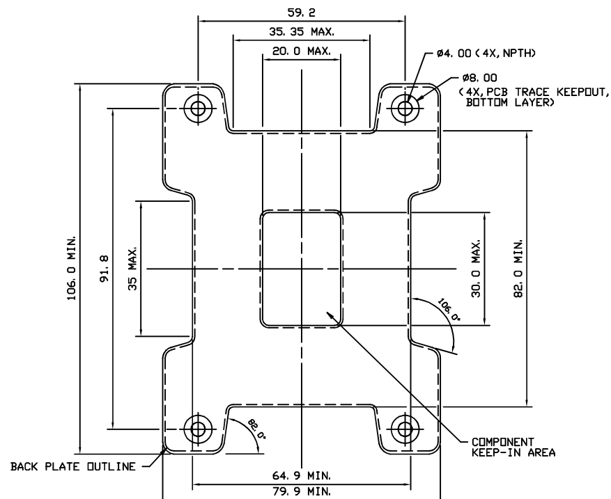
PCB KEEP-OUT ZONE FOR SOCKET SP3 BACK PLATE
