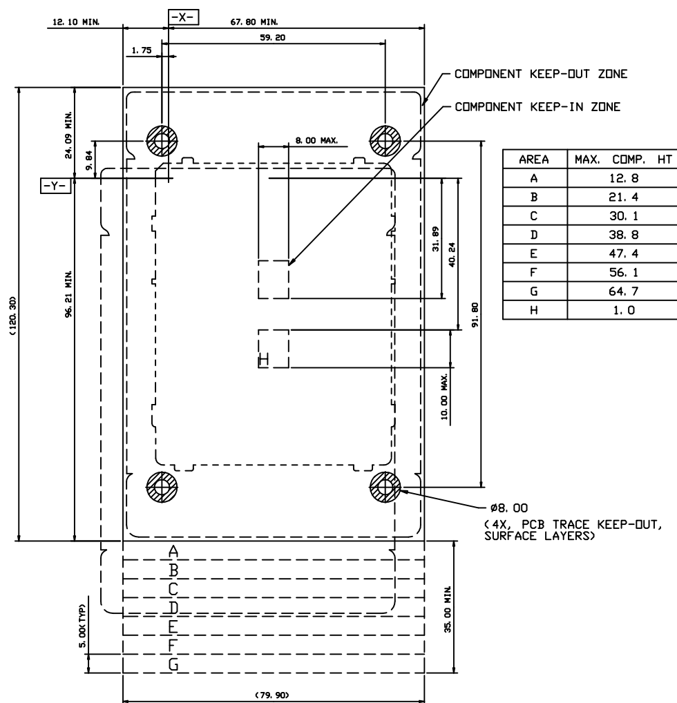
RECOMMENDED PCB KEEPOUT
