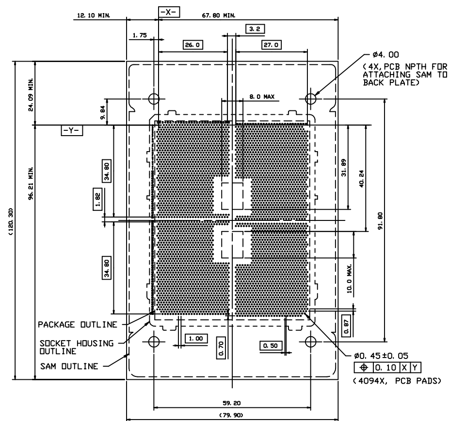
RECOMMENDED PCB PAD LAYOUT
