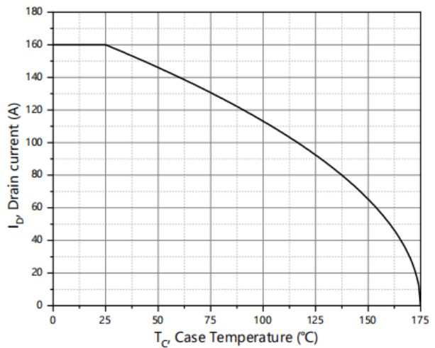
Figure 10. Drain current
