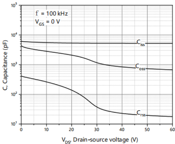
Figure 3. Typ. capacitances
