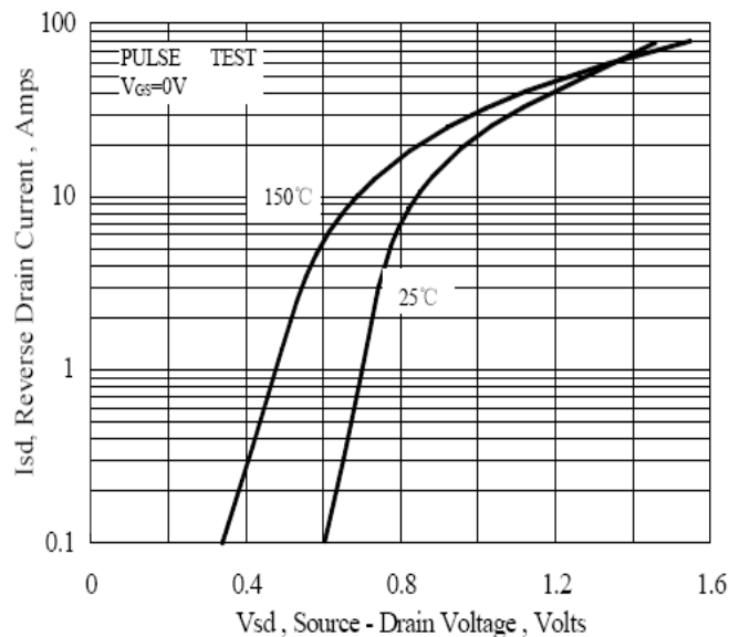
Figure 15 Typical Body Diode Transfer Characteristics
