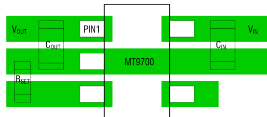
Figure 3. MT9700 Suggested Layout
