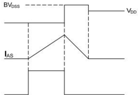
Fig10 EAS Waveform
