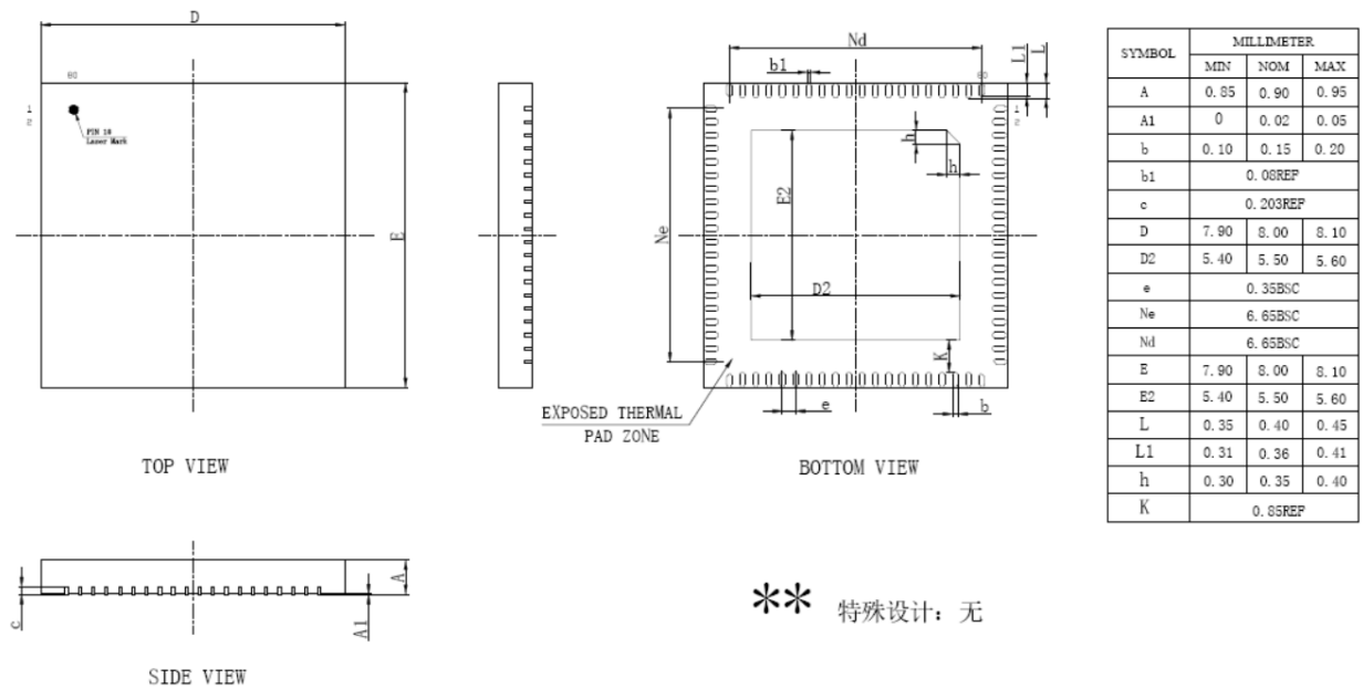
Figure 7.1 – SL6341B QFN80 (8x8) Package
