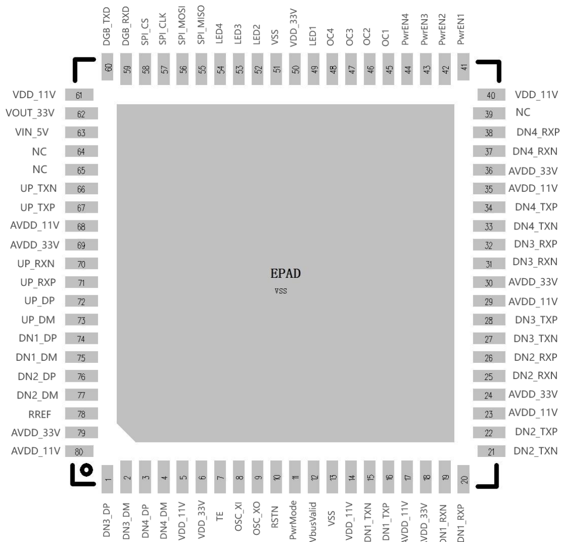
Figure 4.1 – SL6341B QFN80(8x8-0.35) Pin out Diagram
