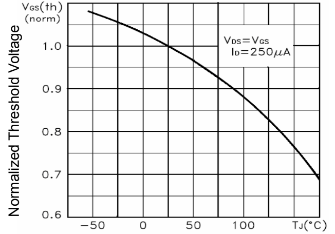
TJ-Junction Temperature(°C) Figure 14 VGS(th) VS Junction Temperature
