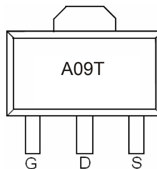
SOT-89 -3L top view
