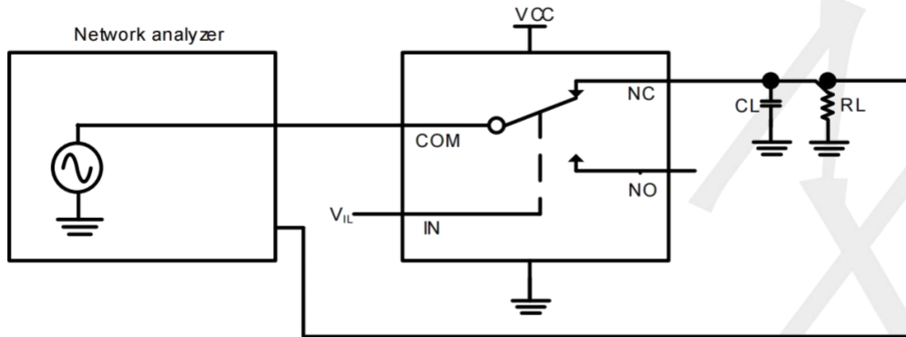
Bandwidth
