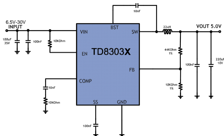
6.5V-30V Input Voltage, 5V Output Voltage Step-Down Converter
