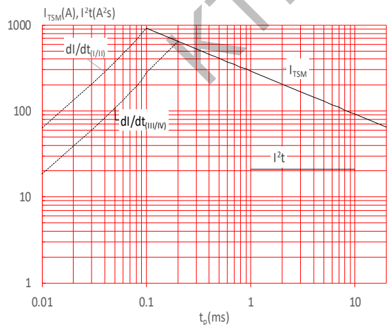
FIG.5: Non-repetitive surge peak on-state current for a sinusoidal pulse with width t_p < 20\text{ms} , and corresponding value of I^2t ( I-II: di/dt < 80\text{A}/\mu\text{s} ; III-IV: di/dt < 40\text{A}/\mu\text{s} )
