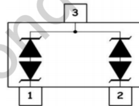
PIN CONFIGURATION
