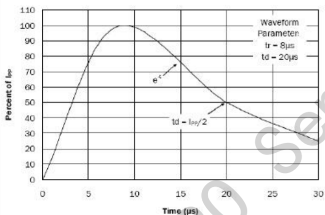
Pulse Waveform
