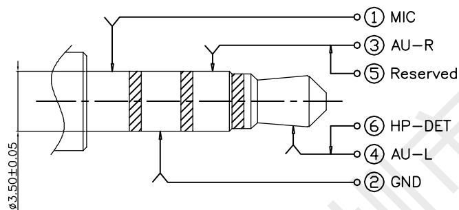
(Ø3.50mm 4 POLE PLUG DETAIL DRAWING)
