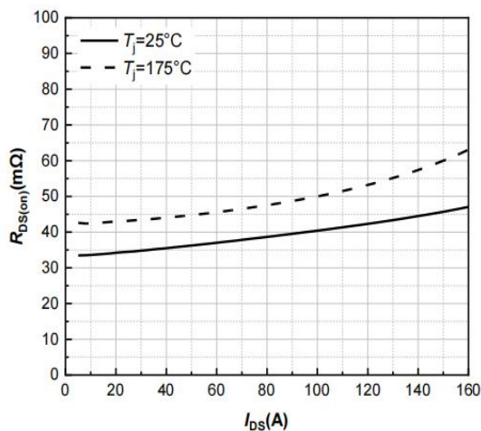
Fig.5 R_{DS(on)} VS I_{DS} (A)
