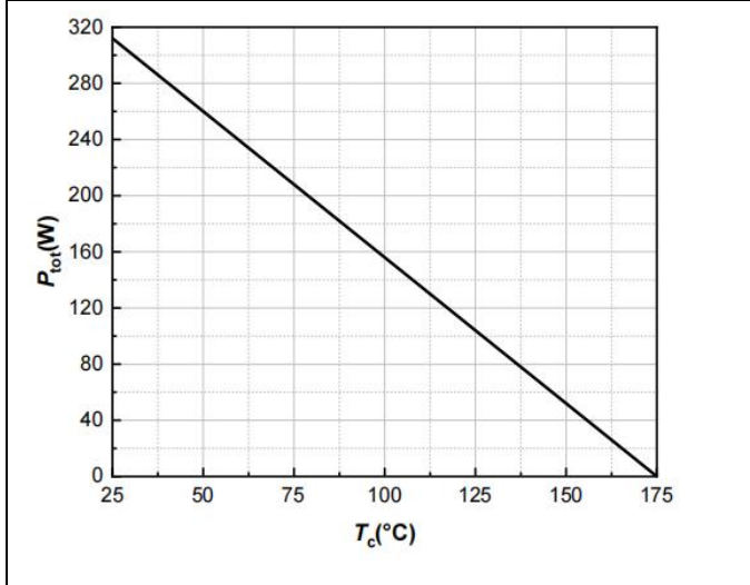
Fig.19 P_{tot} vs T_c(^{\circ}C)
