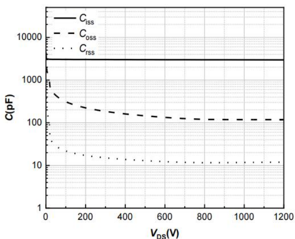
Fig.17 Capacitances vs. Drain-Source
