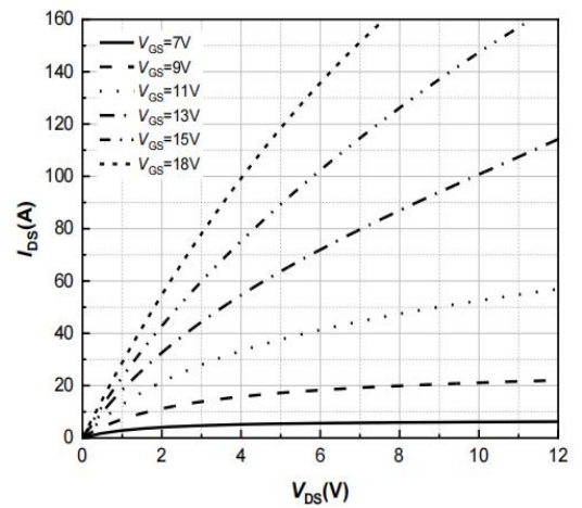
Fig.2 Output Characteristics T_j = 25^\circ\text{C}
