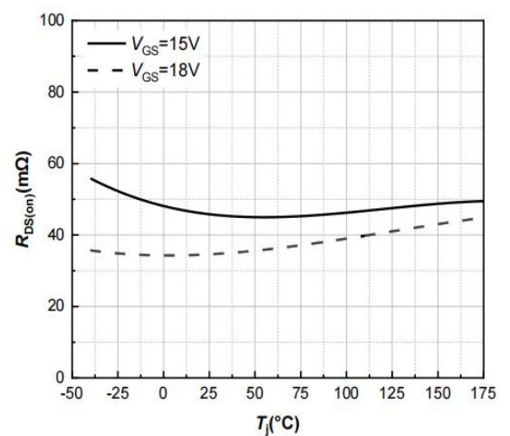
Fig.6 R_{DS(on)} VS T_j ( ^\circ\text{C} )
