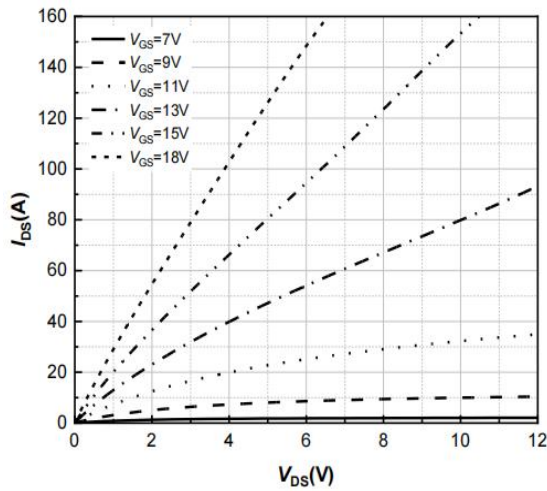
Fig.1 Output Characteristics T_j = -40^\circ\text{C}
