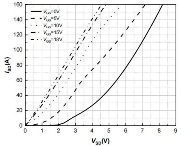
Fig.14. 3rd Quadrant Characteristic T_j = 25^\circ\text{C}
