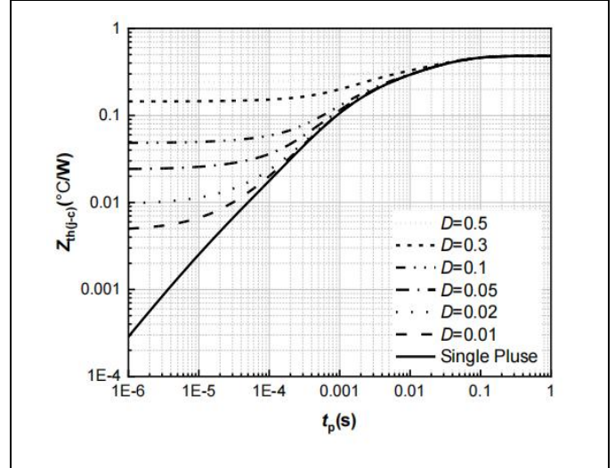
Fig.20 Transient Thermal Impedance
