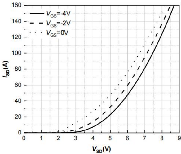
Fig.9 Body Diode Characteristic T_j = 25^\circ\text{C}
