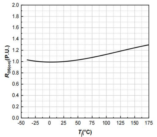
Fig.4 Normalized R_{DS(on)} DS vs. Temperature
