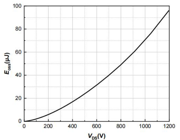
Fig.16 Output Capacitor Stored Energy
