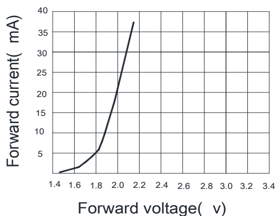
Voltage current relationship
