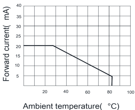
Current and a`mbient temperature
