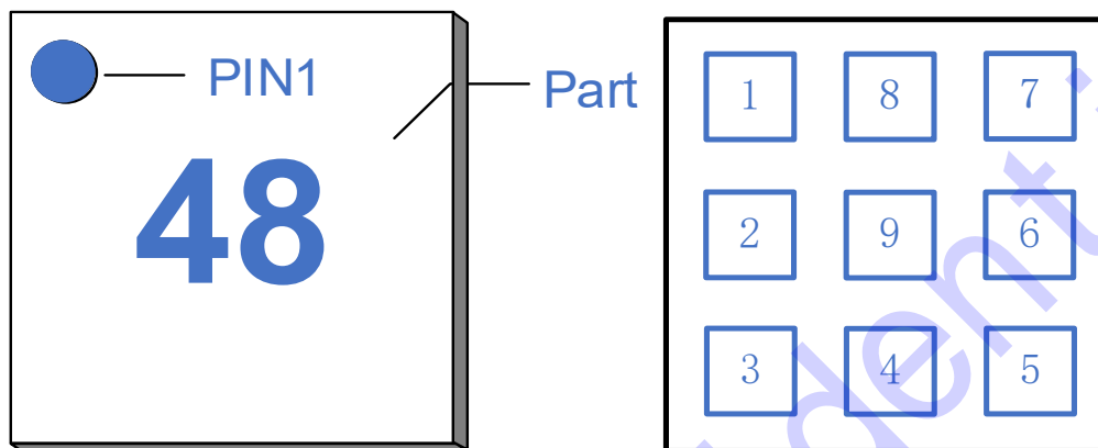
Figure 2 Pin-out Information
