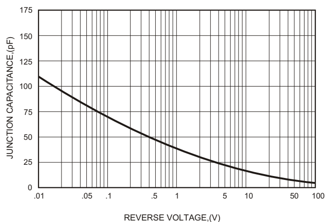
FIG.6-TYPICAL JUNCTION CAPACITANCE
