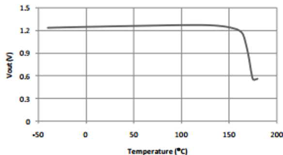
Thermal performance with OTP 1117 A Thermal performance with OTP
