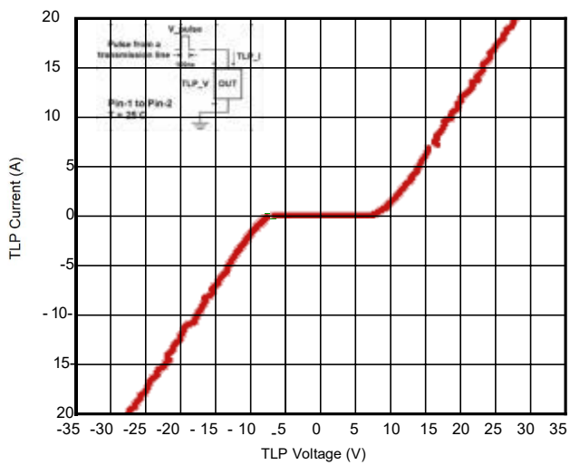
Fig 3. TLP Measurement
