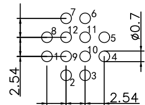
PCB开孔尺寸 PCB cut-out size
