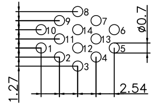
PCB开孔尺寸 PCB cut-out size
