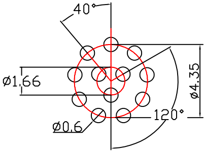
PCB开孔尺寸 PCB cut-out size
