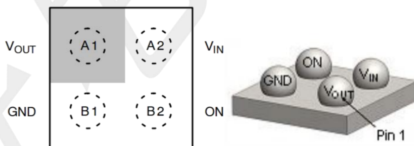
Pin Assignments (Top View)
