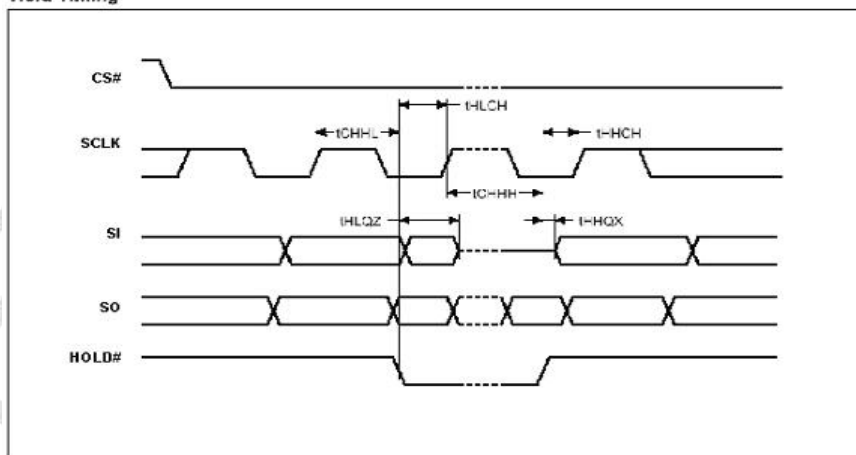
Hold Timing
