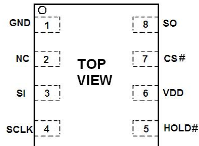
DFN8 2X3
