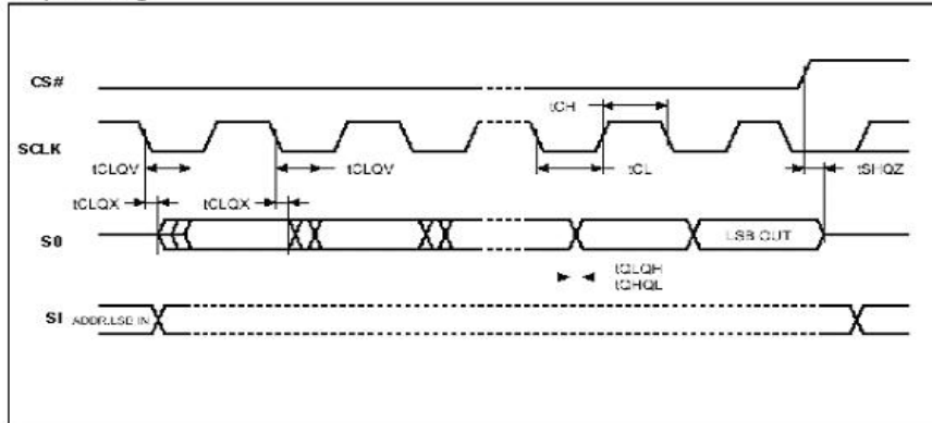
Output Timing
