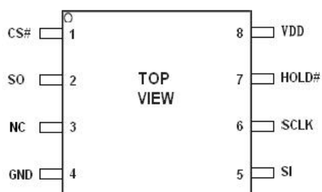
SOP8-B
