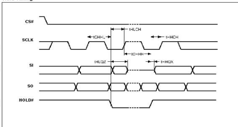
Hold Timing
