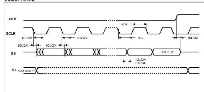
Output Timing
