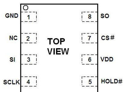
DFN8 2X3
