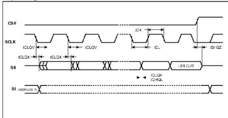
Output Timing
