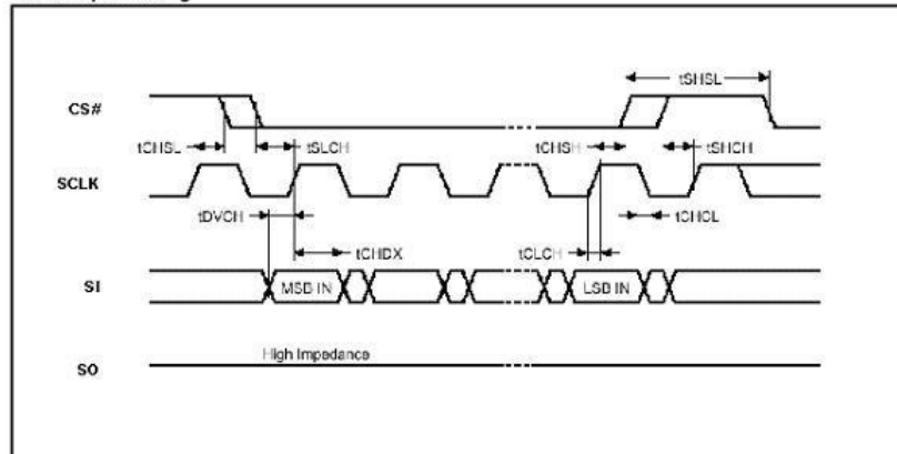
Hold Timing
