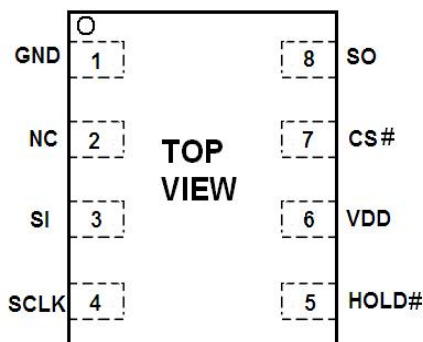
DFN8 2X3
