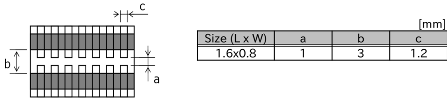
Fig.2: Board of Adhesive Force of Terminal Electrodes, Vibration, and Thermal Shock Tests
