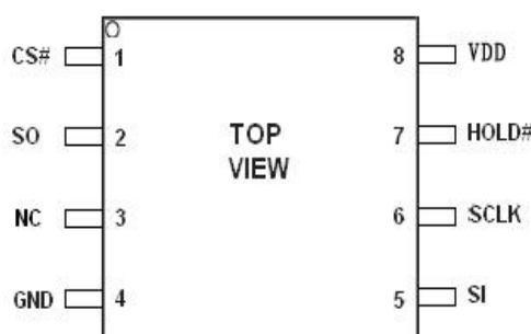
SOP8-B
