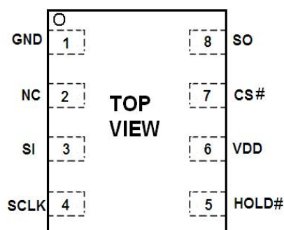
DFN8 2X3
