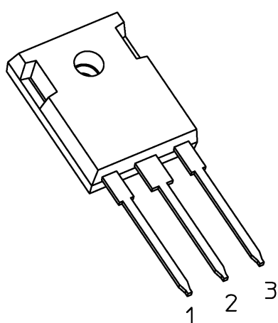
TO-247-3
