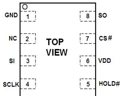
DFN8 2X3
