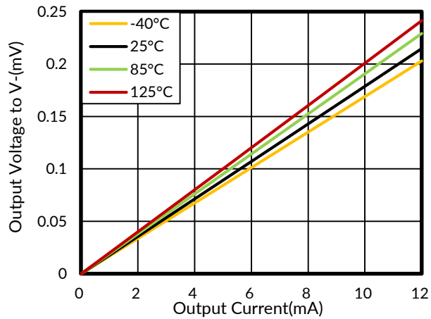
Figure 1. Output Voltage Low vs Output Current, 3V
