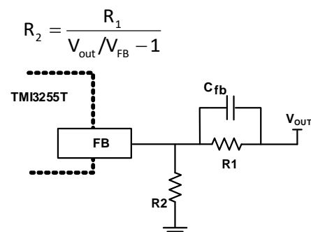
Figure 2. Feedback Network
