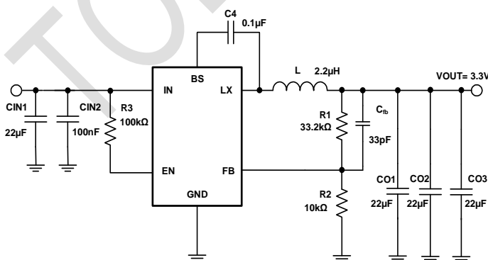
TMI3255T Typical Application Circuits
