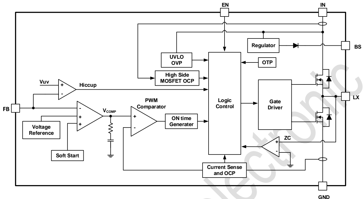
Figure 1. TMI3255T Block Diagram
