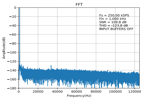
Figure 23. Full-scale FFT (INPUT BUFFERS OFF, External 5V Reference)
