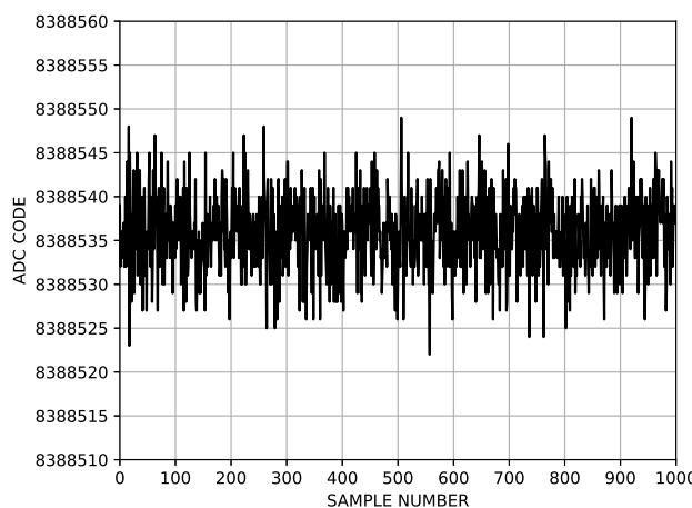
Figure 7. Noise (Analog Input Buffers Disabled, V_{REF} = 5\text{ V} , Output Data Rate = 10 kSPS)
