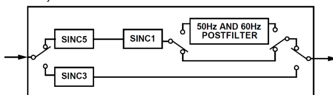
Figure 36. Digital Filter Block Diagram
