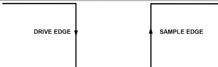
Figure 26. SPI Mode 3 SCLK Edges
