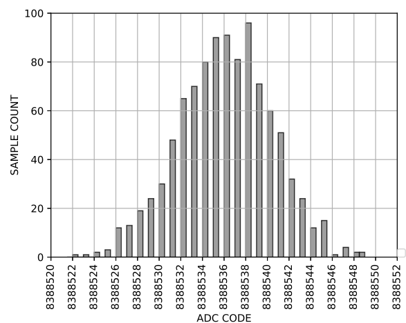
Figure 8. Histogram (Analog Input Buffers Disabled, V_{REF} = 5\text{ V} , Output Data Rate = 10 kSPS)
