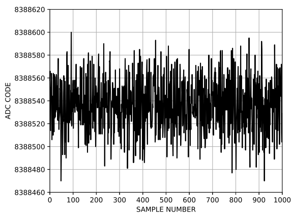
Figure 9. Noise (Analog Input Buffers Disabled, V_{REF} = 5\text{ V} , Output Data Rate = 250 kSPS)
