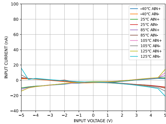
Figure 22. Analog Input Current vs. Input Voltage ( V_{CM} = 2.5\text{ V} )
