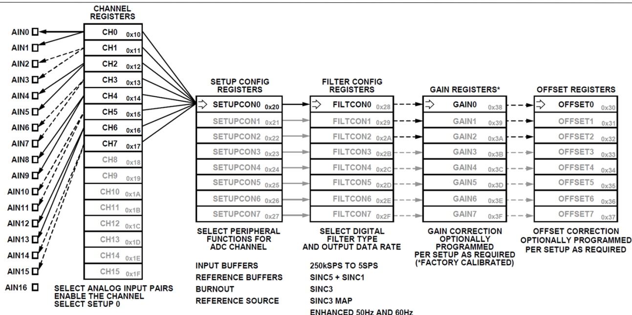
Figure 31. Eight Fully Differential Inputs, All Using a Single Setup (SETUPCON0; FILTCON0; GAIN0; OFFSET0)
