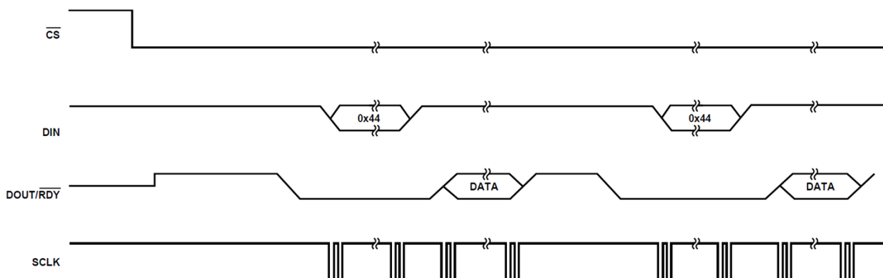
Figure 41. Continuous Conversion Mode
