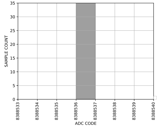
Figure 6. Histogram (Analog Input Buffers Disabled, V_{REF} = 5\text{ V} , Output Data Rate = 5 SPS)
