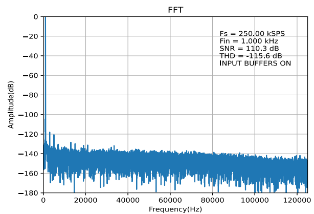
Figure 24. Full-scale FFT (INPUT BUFFERS ON, External 5V Reference)
