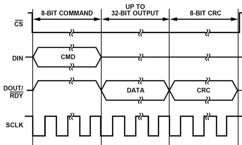
Figure 45. SPI Read Transaction with CRC
