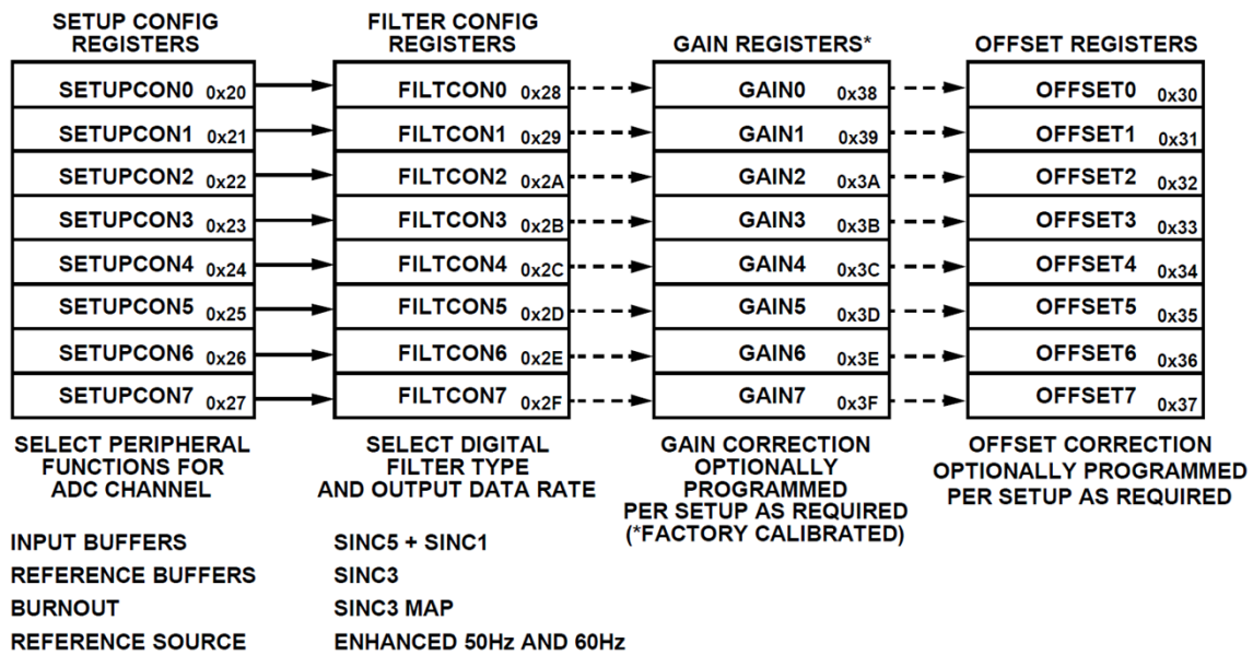
Figure 30. ADC Setup Register Grouping
