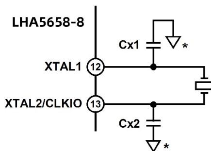
Figure 35. External Crystal Connections
