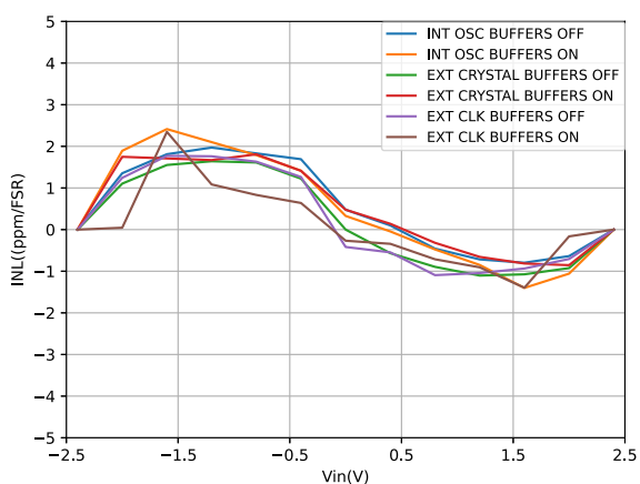
Figure 17. Integral Nonlinearity (INL) vs. V_{IN} (Differential Input, External 2.5 V Reference)
