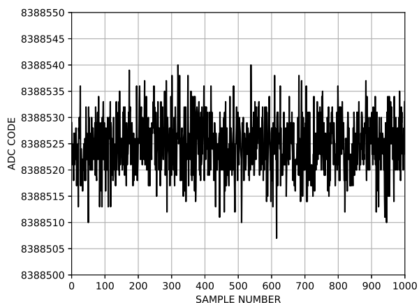
Figure 13. Noise (Analog Input Buffers Enabled, V_{REF} = 5\text{ V} , Output Data Rate = 10 kSPS)
