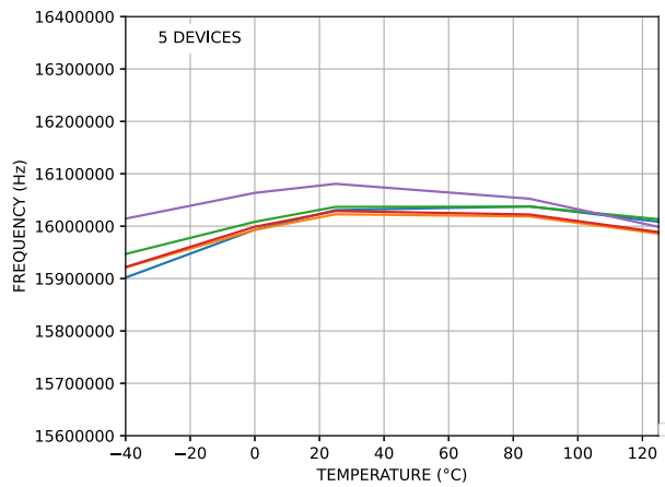
Figure 21. Internal Oscillator Frequency vs. Temperature
