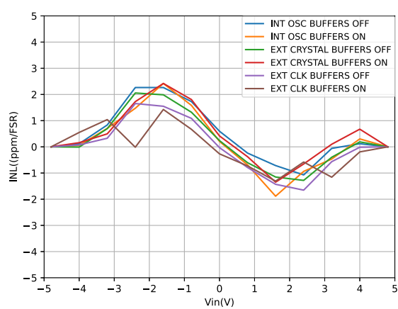
Figure 18. Integral Nonlinearity (INL) vs. V_{IN} (Differential Input, External 5 V Reference)
