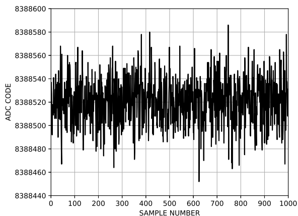
Figure 15. Noise (Analog Input Buffers Enabled, V_{REF} = 5\text{ V} , Output Data Rate = 250 kSPS)
