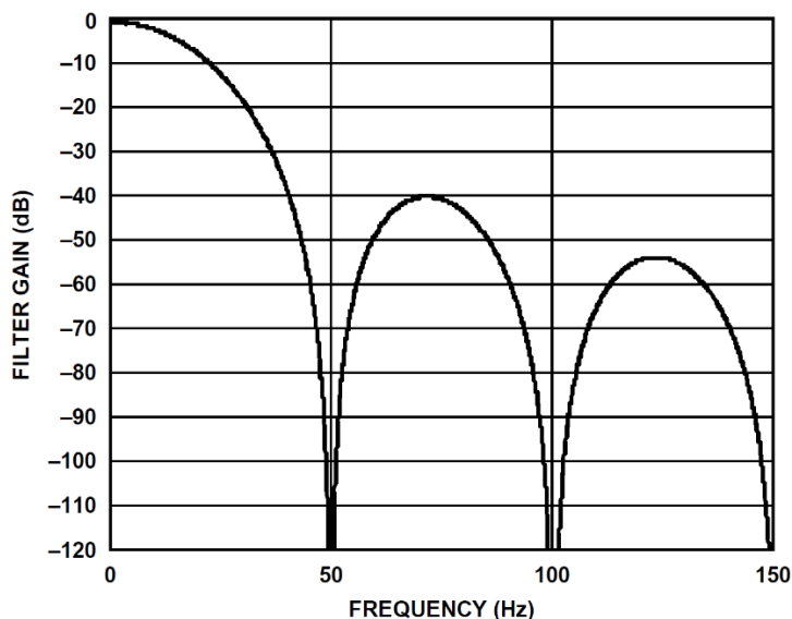
Figure 38. Sinc3 Filter Response
