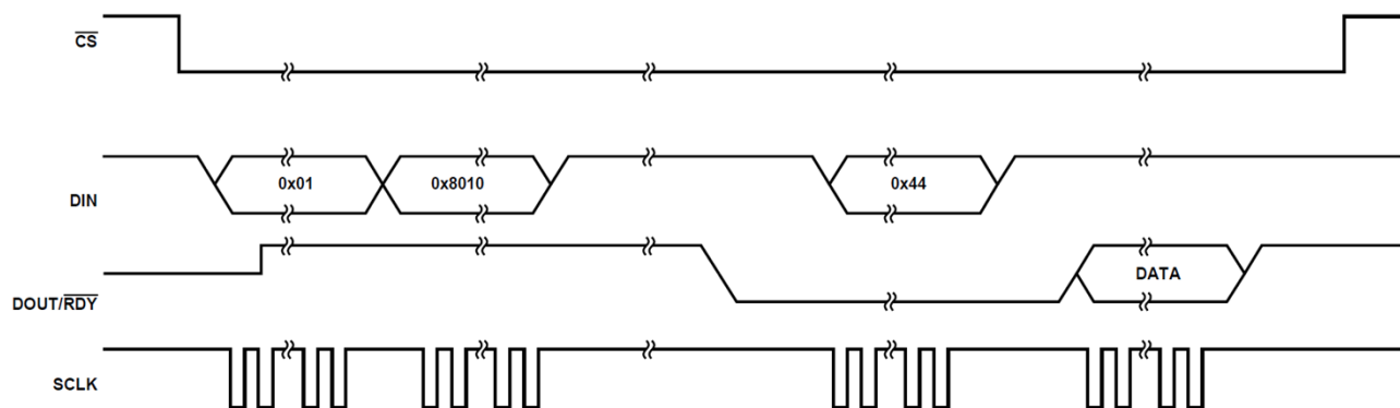
Figure 43. Single Conversion Mode
