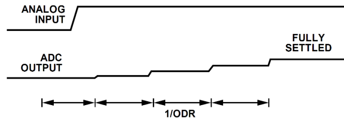
Figure 39. Step Input Without Single Cycle Settling
