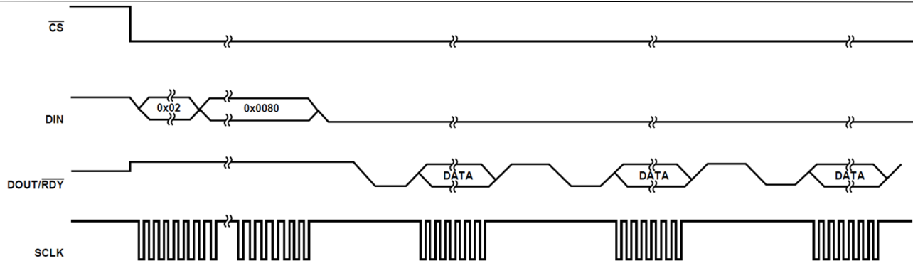
Figure 42. Continuous Read Mode
