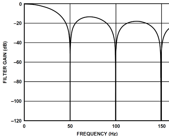
Figure 37. Sinc5 + Sinc1 Filter Response at 50 SPS ODR
