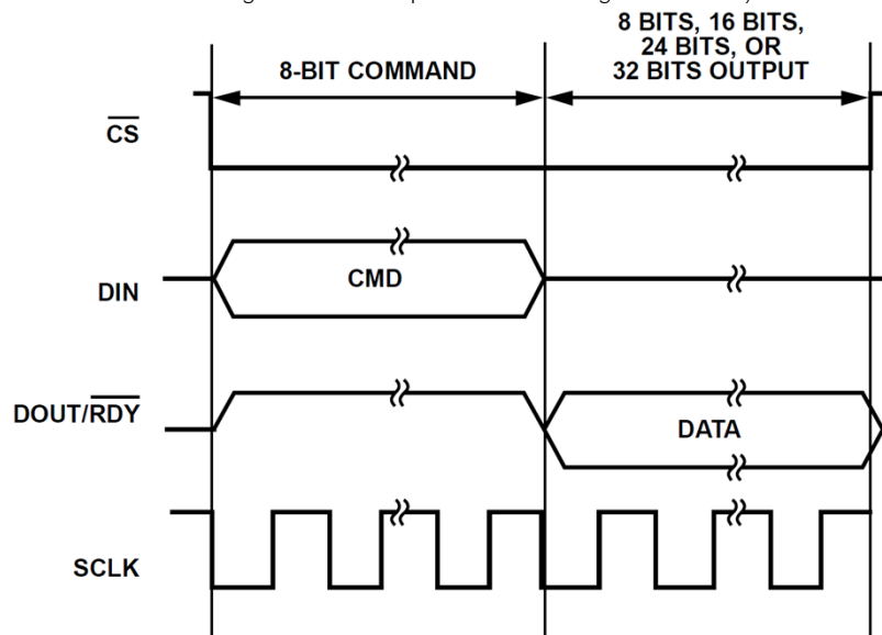
Figure 28. Reading from a Register
