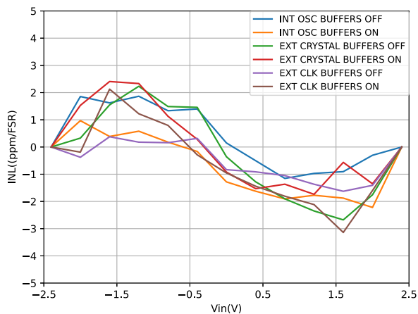
Figure 19. Integral Nonlinearity (INL) vs. V_{IN} (Differential Input, Internal 2.5 V Reference)
