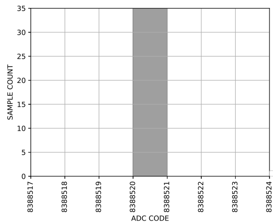
Figure 12. Histogram (Analog Input Buffers Enabled, V_{REF} = 5\text{ V} , Output Data Rate = 5 SPS)
