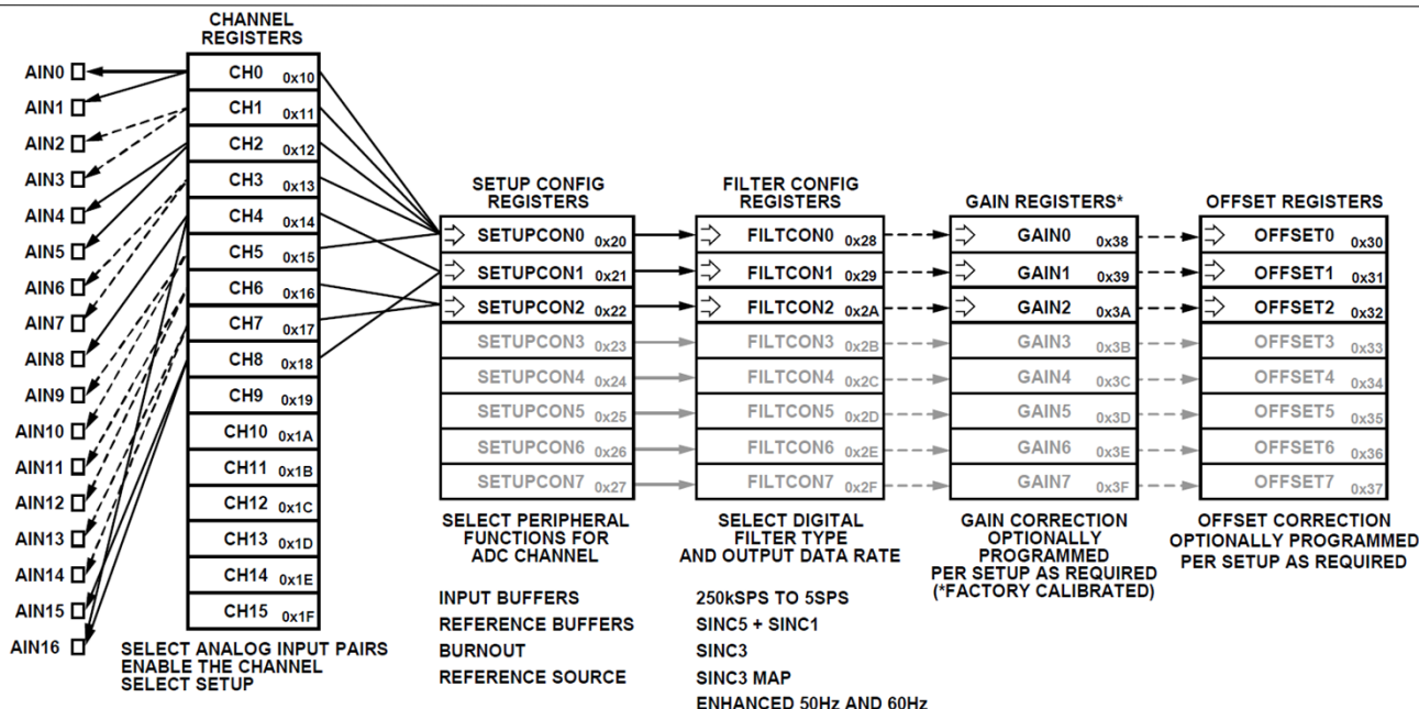
Figure 33. Mixed Differential and Single-Ended Configuration Using Multiple Shared Setups
