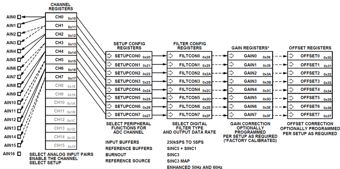
Figure 32. Eight Fully Differential Inputs with a Setup per Channel
