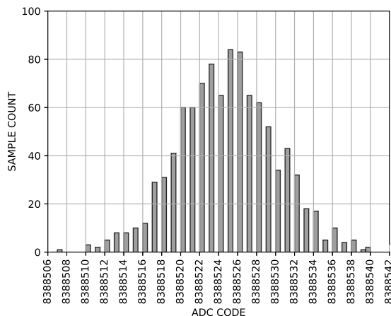
Figure 14. Histogram (Analog Input Buffers Enabled, V_{REF} = 5\text{ V} , Output Data Rate = 10 kSPS)
