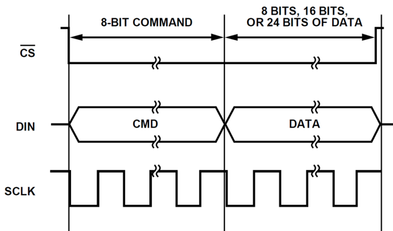
Figure 27. Writing to a Register
