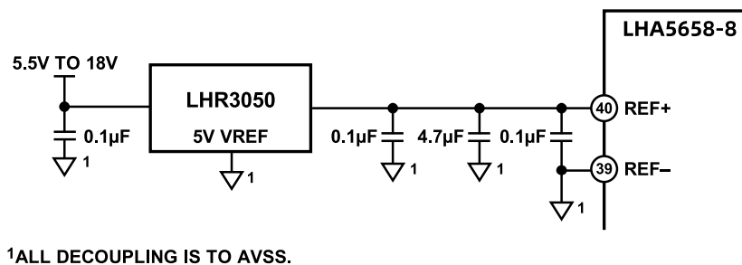
Figure 34. External Reference LHR3050 Connected to the LHA5658-8 Reference Pins
