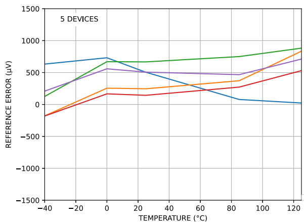
Figure 20. Absolute Reference Error vs. Temperature
