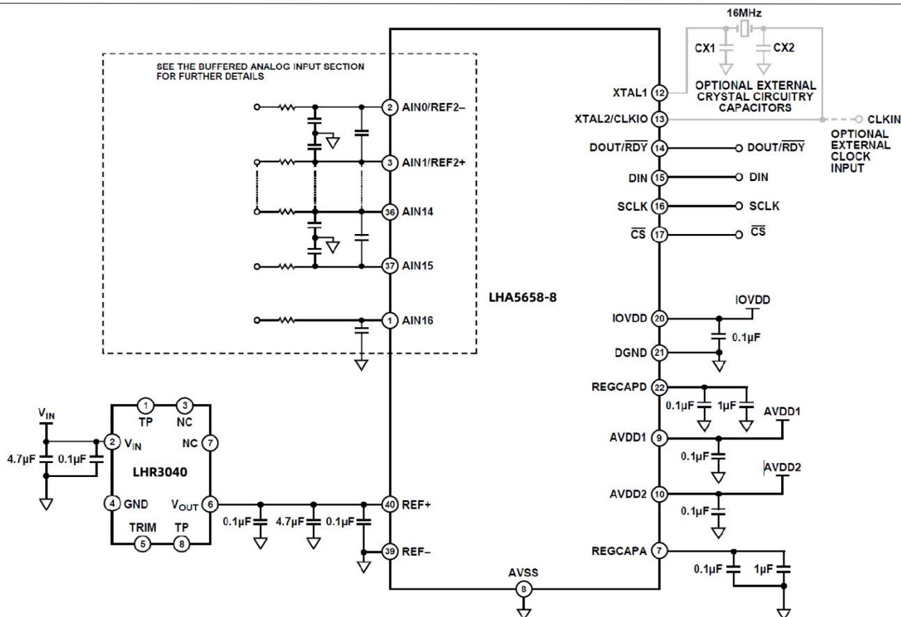
Figure 25. Typical Connection Diagram
