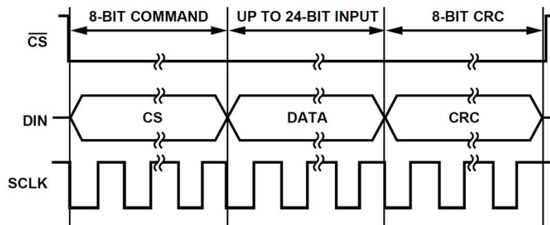
Figure 44. SPI Write Transaction with CRC
