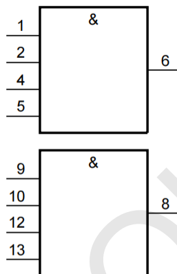
Figure 2. IEC logic symbol
