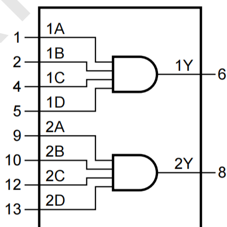
Figure 4. Functional diagram
