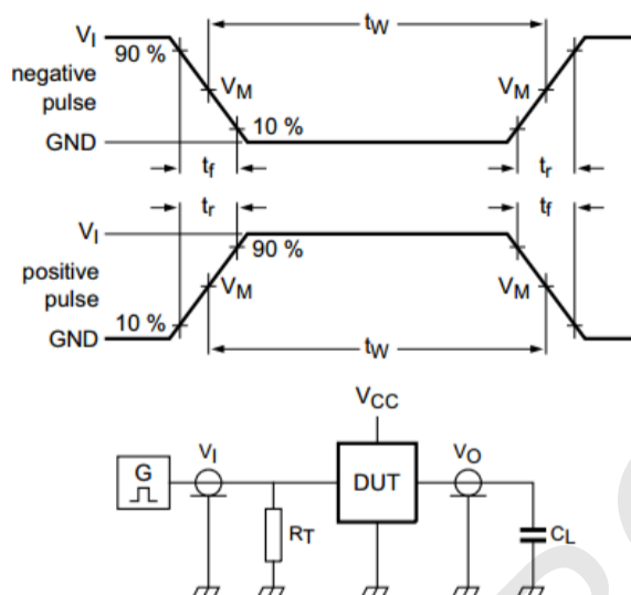
Figure 5. Test circuit for measuring switching times
