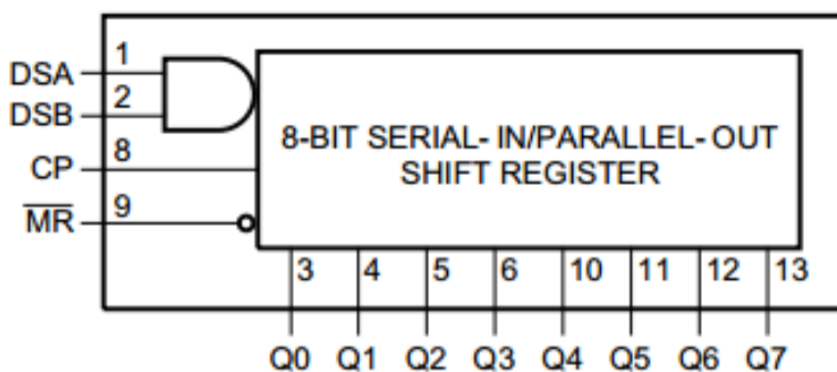
Figure 3. Logic diagram
