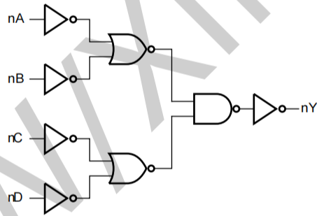
Figure 2. Logic diagram (one gate)
