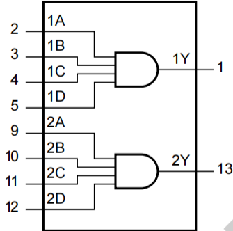
Figure 1. Functional diagram
