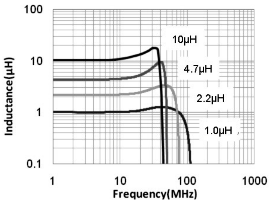
Inductance vs. Frequency Characteristics
