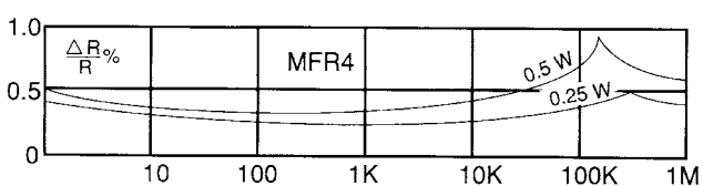
Graph 2 – Load for 1000 hours at 70°C: maximum changes
