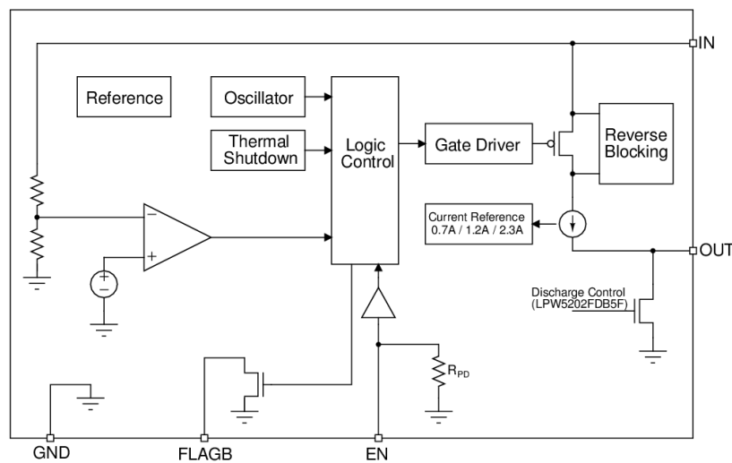
Figure 3. Internal Block Diagram (LPW5202F)
