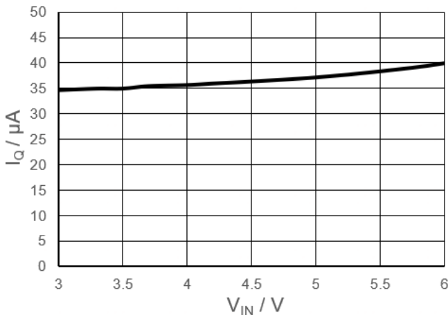
Figure 6. Quiescent Current vs Input Voltage (C IN =C OUT =1μF, V EN = V IN , no load, T A = 25 °C)
