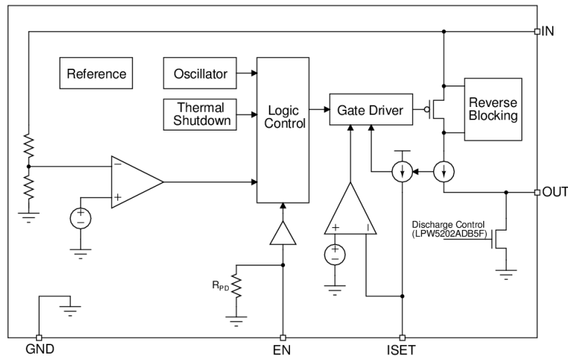
Figure 2. Internal Block Diagram (LPW5202A)
