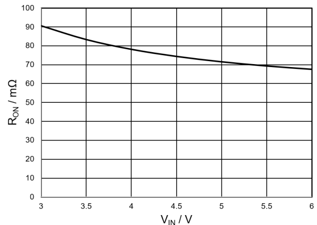
Figure 9. On-Resistance vs Input Voltage (V EN = V IN , I LOAD = 1A, T A = 25 °C)
