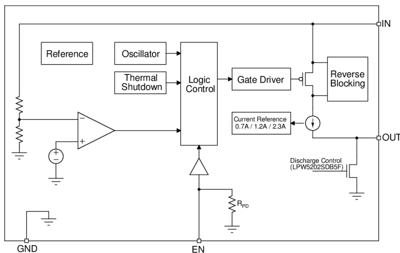
Figure 4. Internal Block Diagram (LPW5202S)
