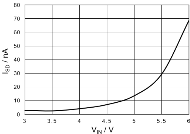
Figure 8. Shutdown Current vs Input Voltage (C IN =C OUT =1μF, V EN = 0V, no load, T A = 25 °C)
