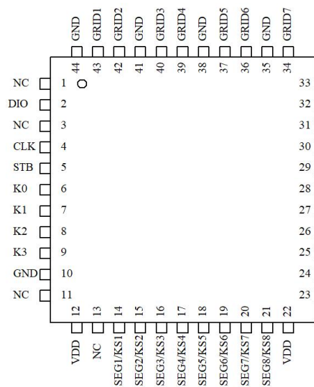
HTM1629F-TD 44LQFP
