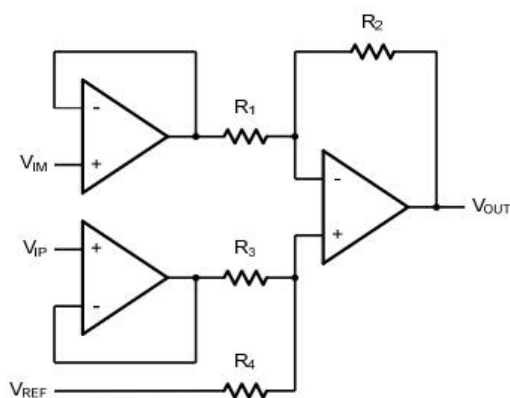
Figure 6. Instrument Amplifier
