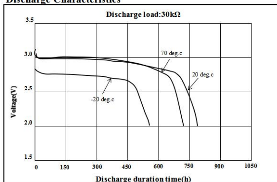
Discharge Characteristics
