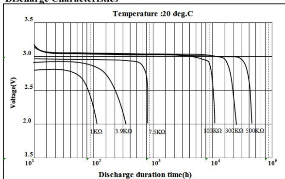
Discharge Characteristics
