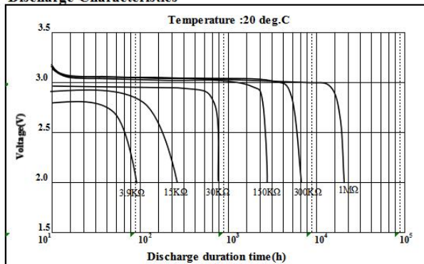
Discharge Characteristics
