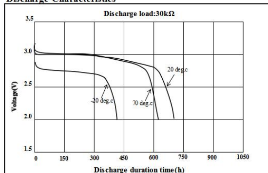
Discharge Characteristics
