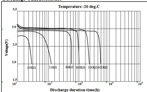
Discharge Characteristics
