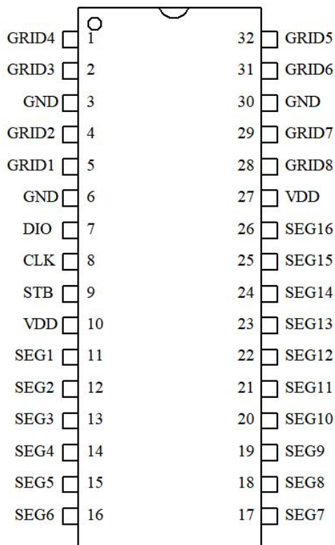
HTM1629A-TD 32SOP
