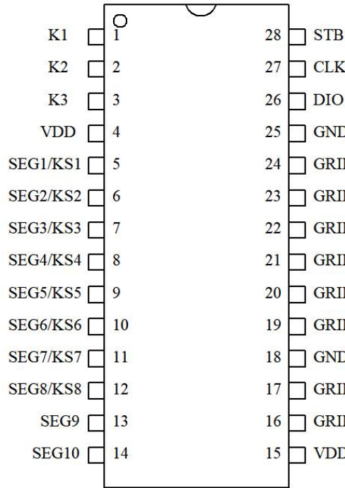
HTM1638-TD 28SOP/28SSOP
