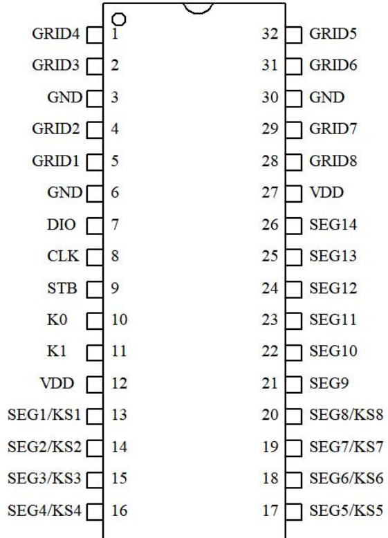
HTM1629B-TD 32SOP
