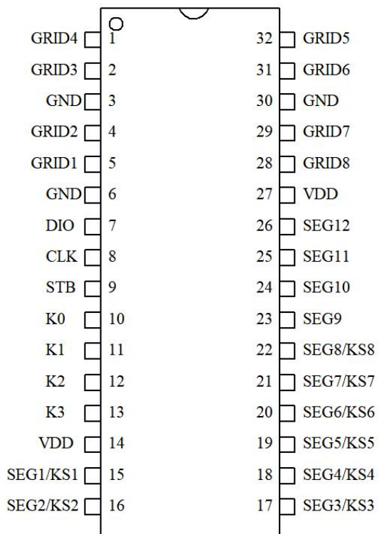
HTM1629D-TD32SOP
