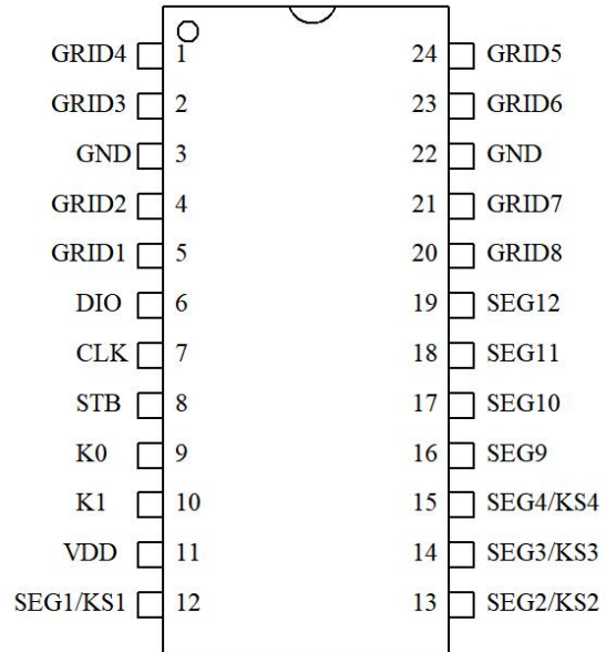
HTM1639-TD 24SOP/24SSOP
