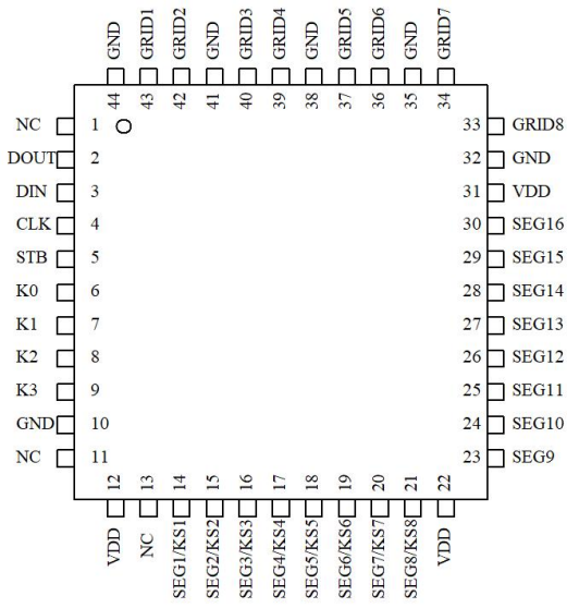
HTM1629E-TD 44LQFP
