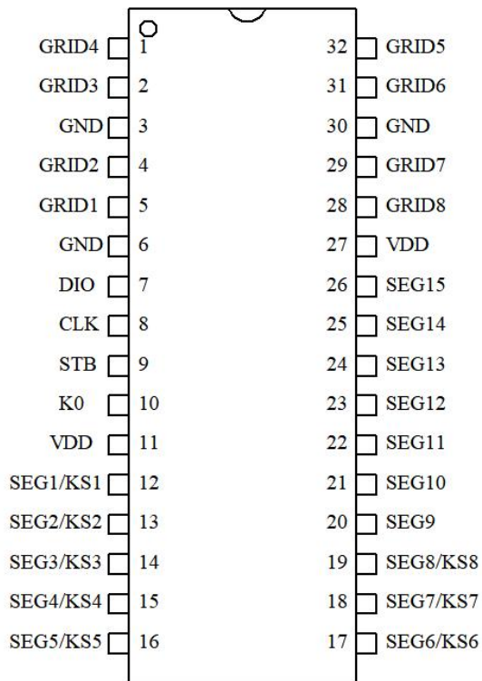
HTM1629C-TD32SOP
