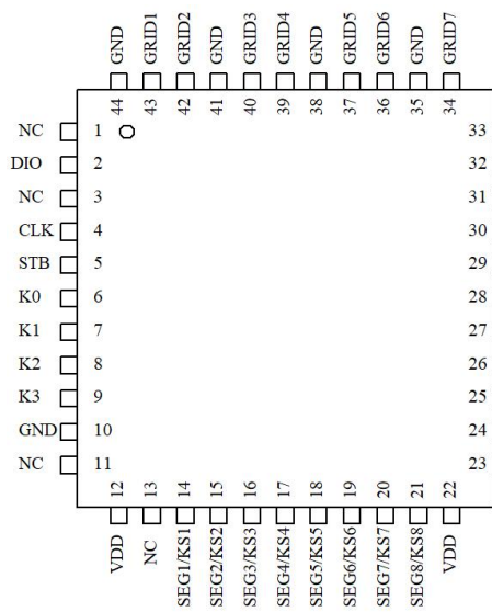
HTM1629-TD 44LQFP
