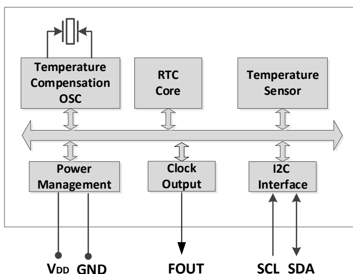
Figure 1. Block Diagram
