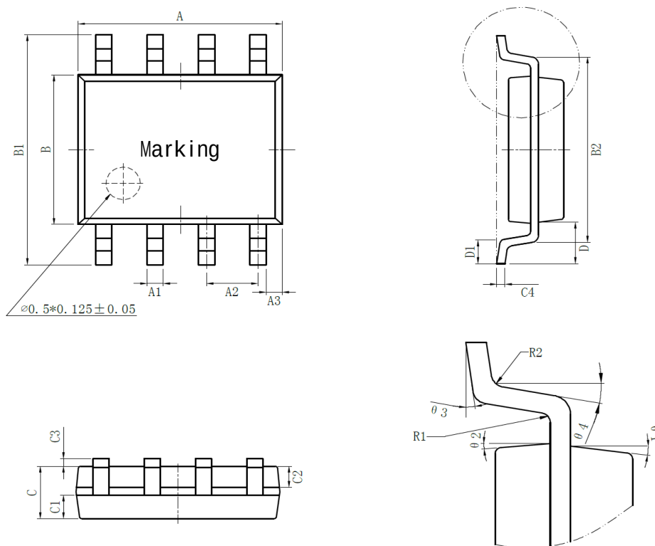
Figure 4. Dimension
