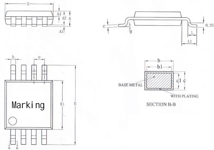
TSSOP8 Dimension and Mark
